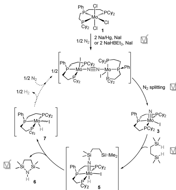
Scheme 3. Potential four-step homogeneous catalytic cycle for the functionalization of \text{N}_2 using bis(silane) built on the three stoichiometric steps presented herein.
